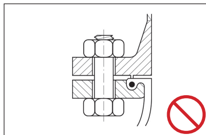
Fig. 3 Do not use flange with tongue or groove which will damage the rubber.
