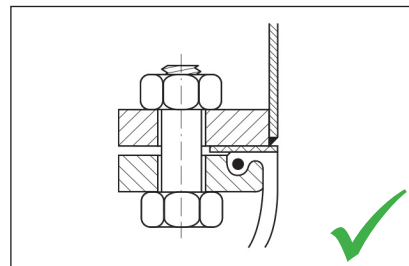
Fig. 4 Flange provided with flat sealing gasket to protect the rubber surface.
