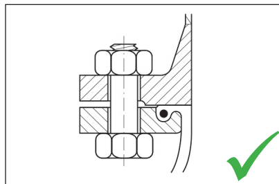
Fig. 2 Flange provided with smooth sealing surface
