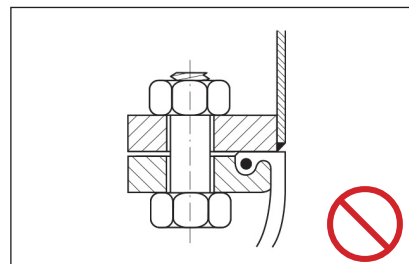
Fig. 5 Sharp edge pipe ends will damage the rubber face.
