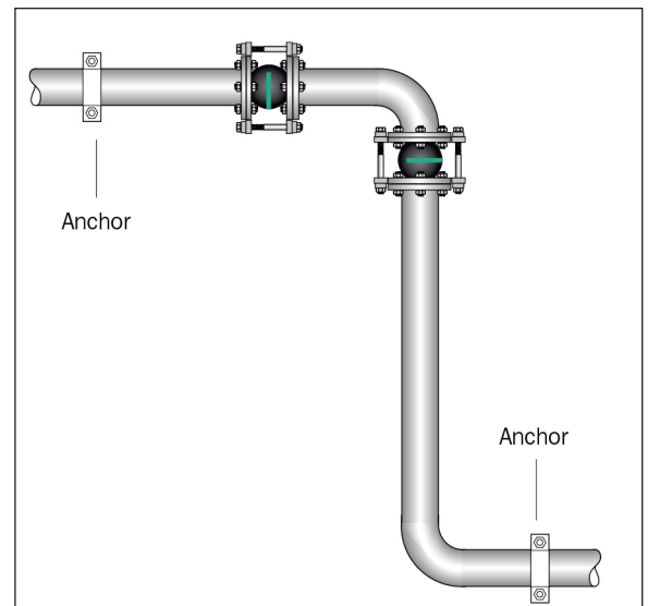
Arrangement with lateral expansion joints.
